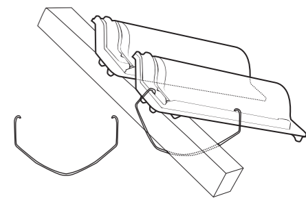
f) clip 416001 for curved and flat interlocking tiles
