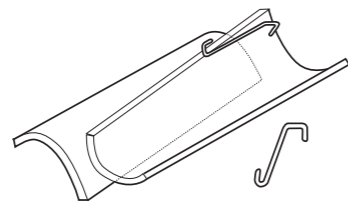
b) clip for cover tiles with hole
