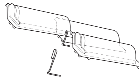
d) clip 409002 for curved and flat interlocking tiles
