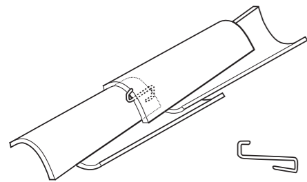
a) clip for cover tiles
