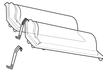
c) clip 455002 for curved interlocking tiles
